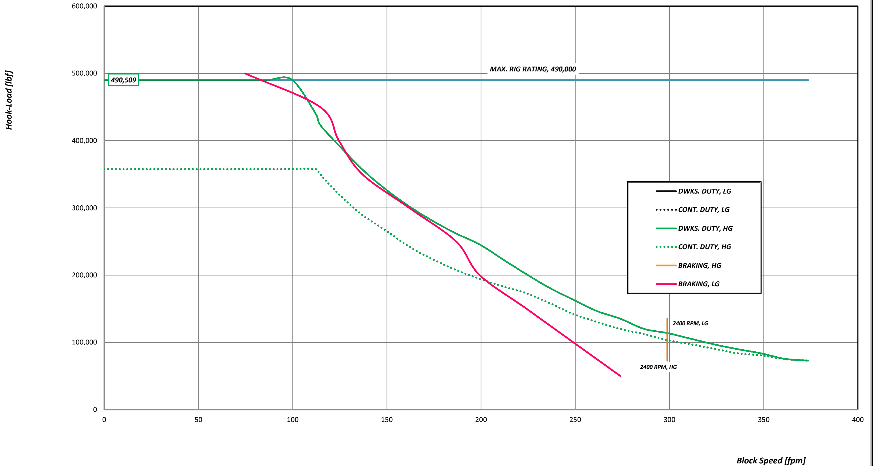
Hook-Load vs. Block-Speed, 8 Lines, LS Ratio = 8.51, HS Ratio = 8.51, Motor-Capacity Limited
