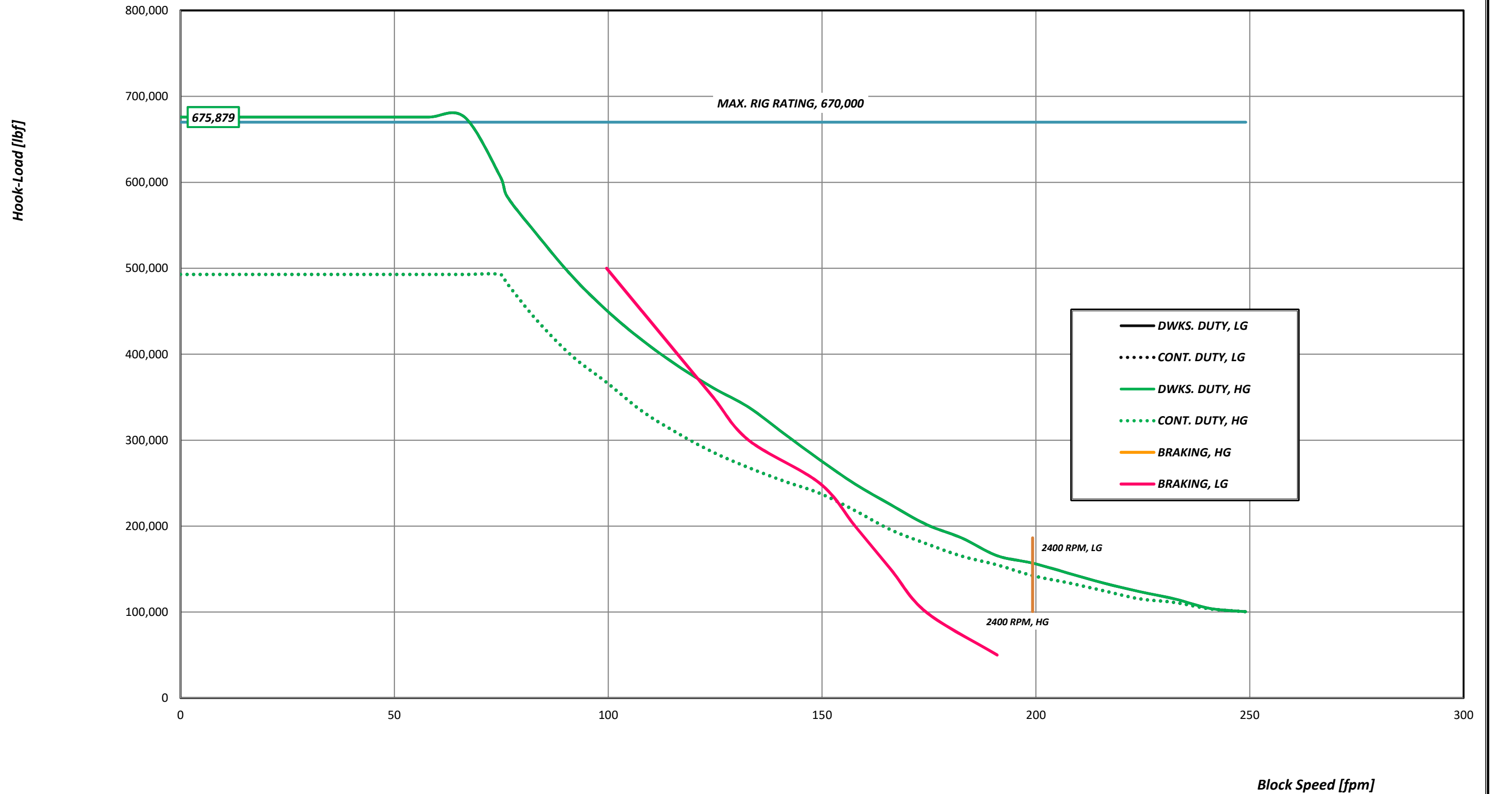
Hook-Load vs. Block-Speed, 12 Lines, LS Ratio = 8.51, HS Ratio = 8.51, Motor-Capacity Limited
