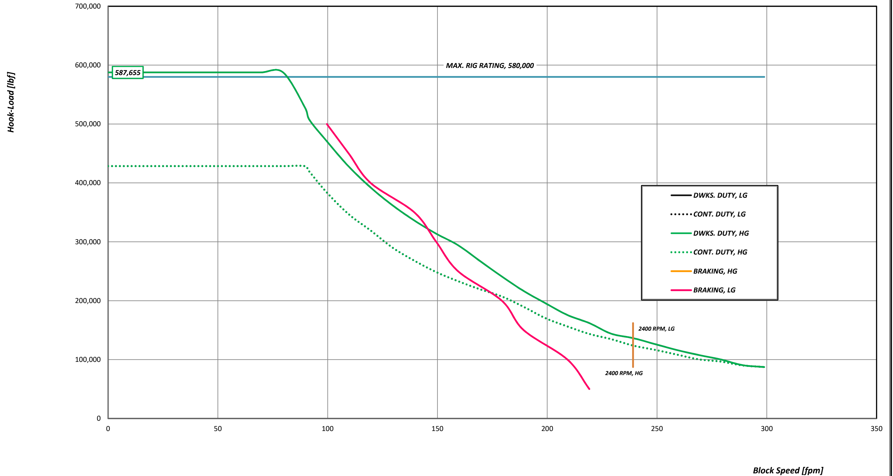
Hook-Load vs. Block-Speed, 10 Lines, LS Ratio = 8.51, HS Ratio = 8.51, Motor-Capacity Limited
